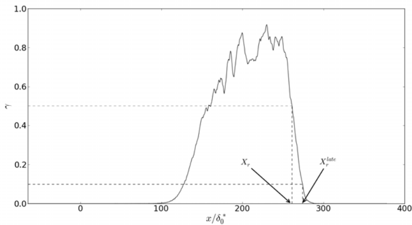
Fig. 2. Probability of reverse flow (averaged over time and z-direction)
