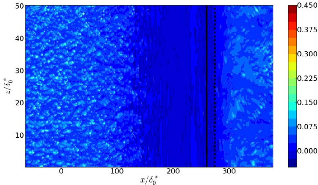
Fig. 6. An instantaneous skin friction field corresponding to the late reattachment event: — mean reattachment line, - - - late reattachment line
