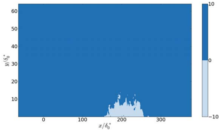
Fig. 3. Time evolution of backflow region ( z \approx 25\delta_0^* )
