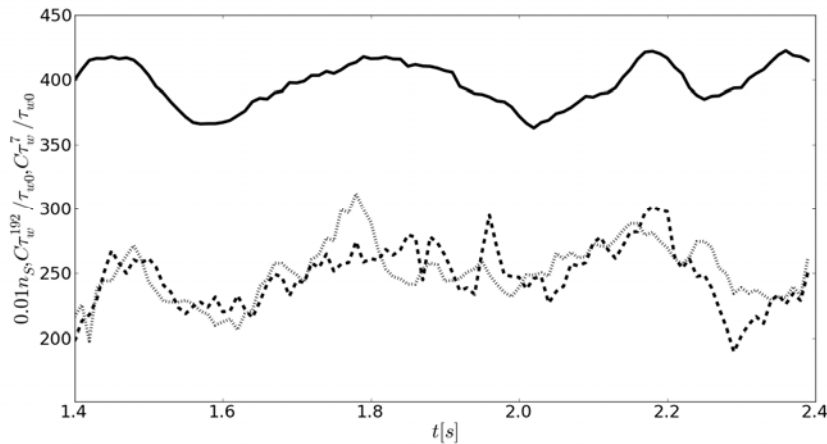
Fig. 7. Time evolution of the following parameters: — total area of the backflow region n_s ; --- instantaneous skin friction averaged over z - direction C\tau_w^{192}/\tau_{w0} (192 points, C=const , x/\delta_0^*=369.2 ); ..... instantaneous skin friction averaged over z - direction C\tau_w^7/\tau_{w0} (7 points, C=const , x/\delta_0^*=369.2 );
