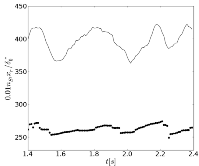
Fig. 5. Time evolution of the total area of the backflow region n_s ( — ) and the pulsation of the instantaneous reattachment point averaged over z -direction x_r/\delta_0^* (•••••)
