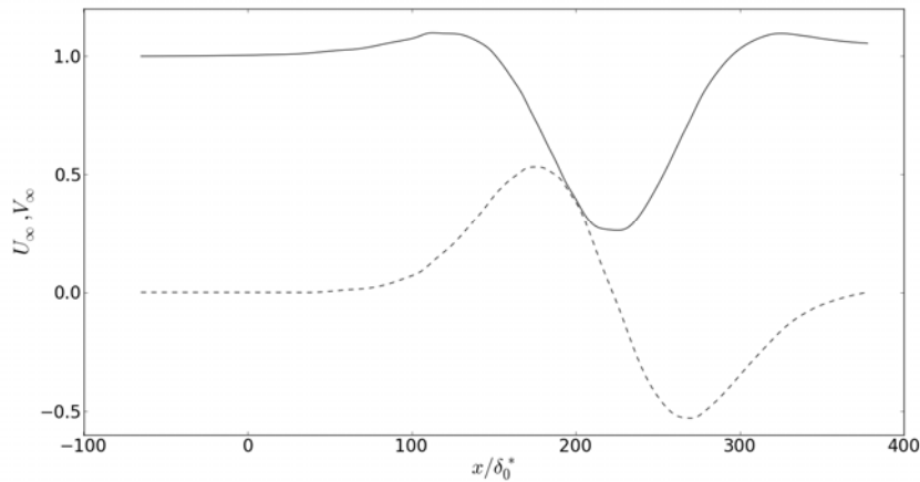
Fig. 1. Free-stream parameters: — U_\infty , --- V_\infty
